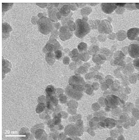
TEM of Zircox™ 3Y-15 (primary powder)
